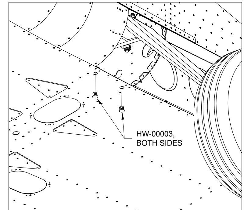
FIGURE 3: DOME PLUG INSTALLATION
